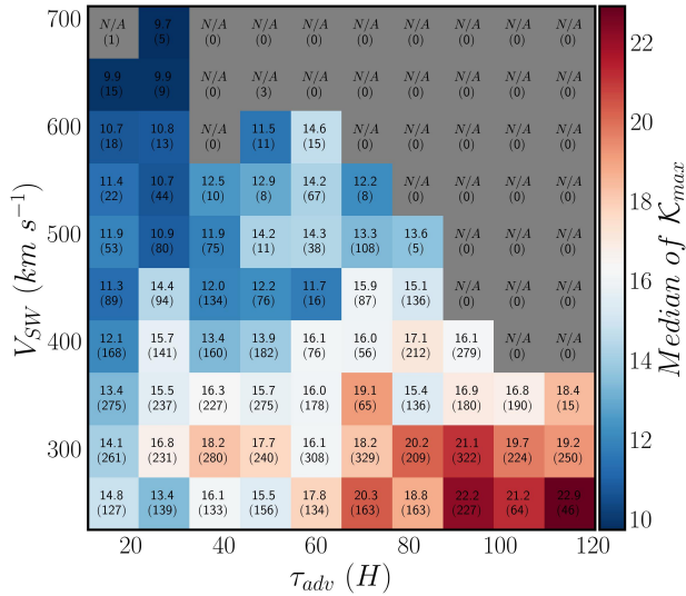
Figure 11. (a) Scale-dependent kurtosis of the magnetic field as a function of solar wind speed V_{SW} and SW advection time \tau_{adv} . The numbers indicate the median value of kurtosis within each bin.
