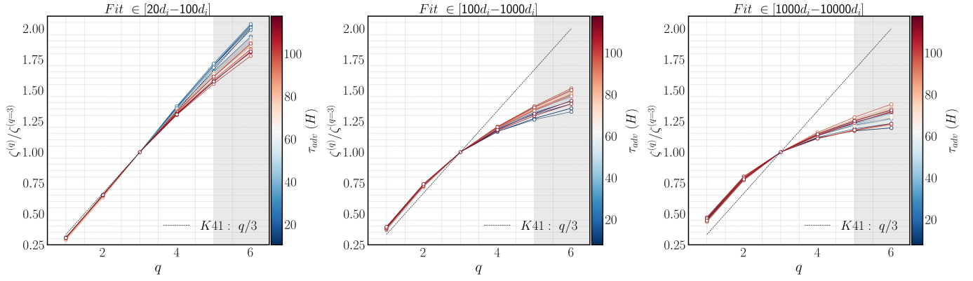
Figure 4. Normalized scaling exponents \zeta(q)/\zeta(3) vs. q , as a function of advection time \tau_{adv} . Each line represents the average of 100 intervals that fall within the same \tau_{adv} bin. The scaling exponents have been obtained by applying a power-law fit on the structure functions ( S_B^q(\ell) ) within three different spatial ranges: (a) [20d_i, 100d_i] , (b) [100d_i, 1000d_i] , (c) [1000d_i, 10000d_i] . The K41 linear scaling is also shown with the black dashed line in all panels. The shaded area has been included to indicate moments that are not determined with reliable accuracy.
