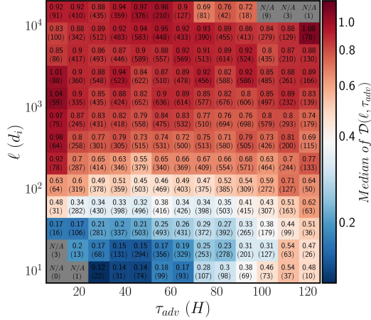
Figure 5. To further quantify the divergence from the linear scaling predicted by the K41 theory of isotropic turbulence, z_{k41}^{(q)} = q/3 , and as a measure of intermittency at a given scale, the quantity \mathcal{D}(\ell, \tau_{adv}) = (\sum (z_{(q=3, \ell)}^{(q, \ell)} - z_{k41}^{(q)})^2)^{1/2} is presented. The data points were binned according to \ell , and \tau_{adv} , and the median value inside each bin was calculated, which is reflected in the colors and written in the plot. The bracketed numbers in the plots are the number of data points inside each bin. Note that bins, including less than 10 data points, were discarded.
