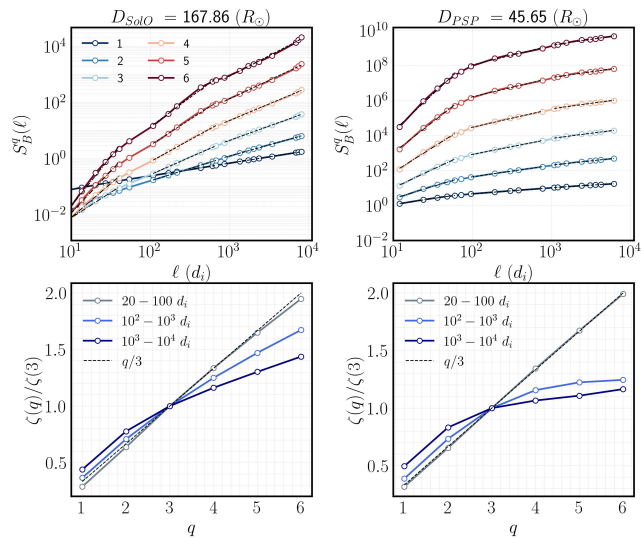
Figure 3. (a) Structure functions for \delta\mathbf{B} , as a function of spatial lags in units of the ion inertial length d_i , S_B^q(\ell) . Power-law fits applied to S_B^q(\ell) , in the range (a) 20 - 10^2 d_i , (b) 10^2 - 10^3 d_i (c) 10^3 - 10^4 d_i are shown as a dashed-dotted and dashed line respectively. (b) The normalized resulting scaling exponents \zeta(q)/\zeta(3) , estimated from Fig. ref:fig:funcsa as a function of q . The K41 ( q/3 ) linear scalings is also shown for comparison.
