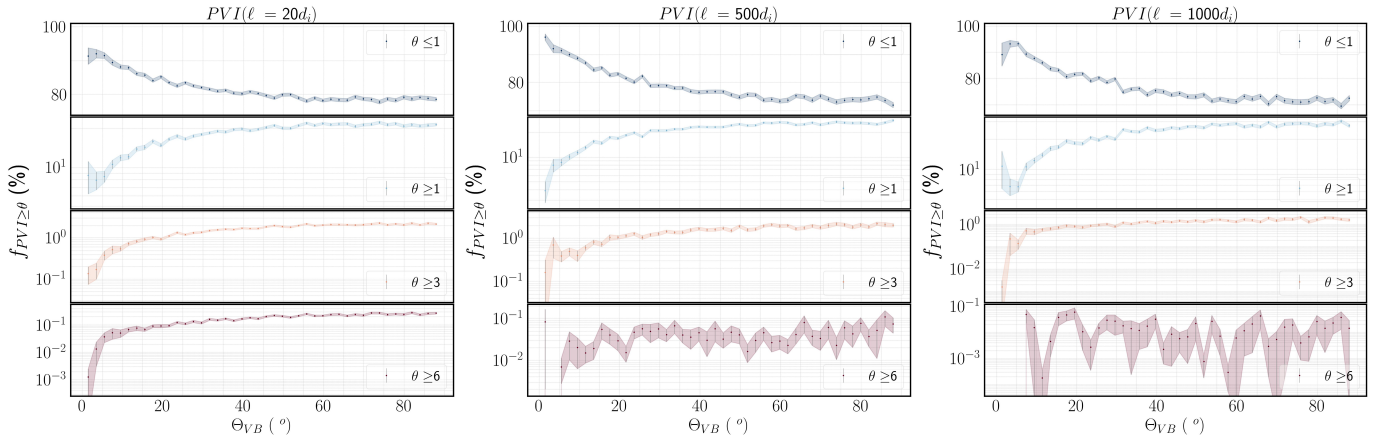
Figure 8. Binned mean of the fraction of PVI events f_{PVI \geq \theta} (%), where \theta = 1, 3, 6 as a function of the angle between solar wind and background magnetic field \Theta_{VB} . Three different lags are considered ( \ell = 1000, 500, 20 d_i ). A total number of n = 45 bins have been used.
