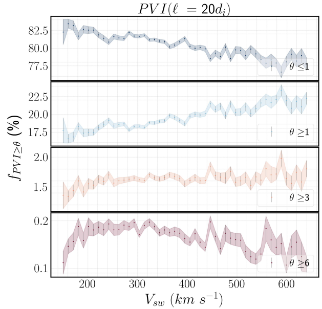
Figure 12. Fraction of datapoints with PVI value exceeding a given threshold, f_{PVI \geq \theta} , where \theta = 1, 3, 6 as a function of solar wind speed, V_{SW} .
