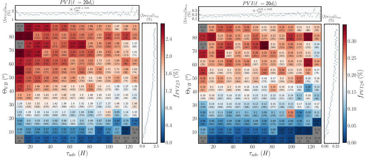
Figure 9. Binned mean of the fraction of datapoints with PVI value exceeding a given threshold, f_{PVI \geq \theta} , where \theta = 3 (left panel) and \theta = 6 (right panel) shown as a function of advection time \tau_{adv} and \Theta_{VB} angle. The PVI timeseries was estimated with a lag, \ell = 20 d_i . The top subplot shows the averaged fraction of coherent structures, over \Theta_{VB} , \langle f_{PVI \geq \theta} \rangle_{\Theta_{VB}} . Power-law fits are also shown as black-dashed lines. Similarly, the right subplot shows the averaged fraction over \tau_{adv} , \langle f_{PVI \geq \theta} \rangle_{\tau_{adv}} .
