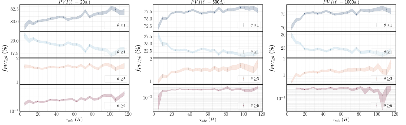
Figure 6. Binned mean of the fraction of datapoints with PVI value exceeding a given threshold ( f_{PVI \geq \theta} , where \theta = [1, 3, 6] ) shown as a function of advection time \tau_{adv} , different thresholds are shown in different colors. Three spatial lags normalized to the ion inertial length d_i are considered, \ell = 20, 500, 1000 d_i .
