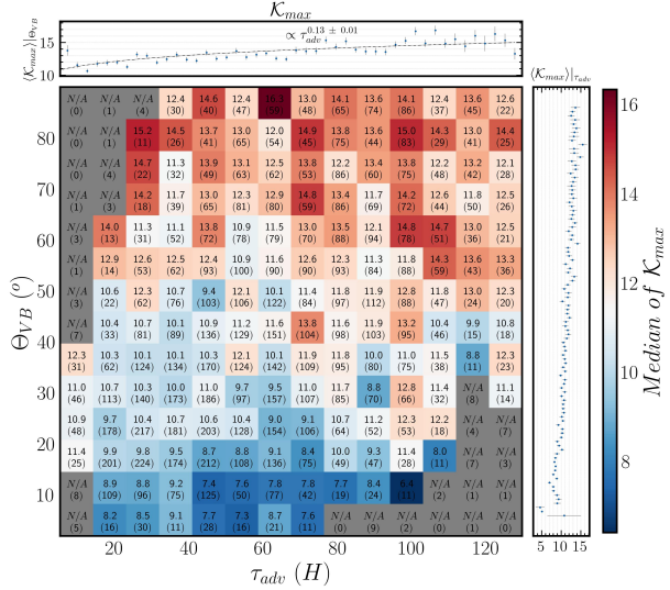
Figure 10. Scale-dependent kurtosis of the magnetic field as a function of \Theta_{VB} and \tau_{adv} . The numbers indicate the median value of kurtosis within each bin. The top subplot shows K_{max} , over \Theta_{VB} , \langle K_{max} \rangle_{\Theta_{VB}} . Power-law fits are also shown as black-dashed lines. Similarly, the right subplot shows the averaged fraction over \tau_{adv} , \langle K_{max} \rangle_{\tau_{adv}} .
