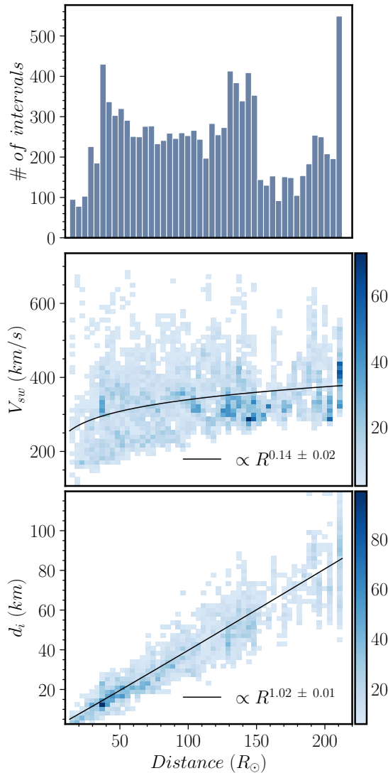
Figure 1. (a) Histogram showing the number of 5-H intervals as a function of heliocentric distance (b) Joint distribution of SW speed V_{sw} vs heliocentric distance ( R ) (c) Joint distribution of ion inertial length d_i vs heliocentric distance ( R ).
